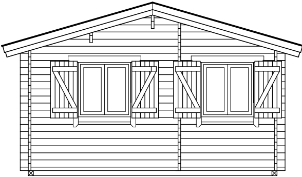
Ansicht -B
