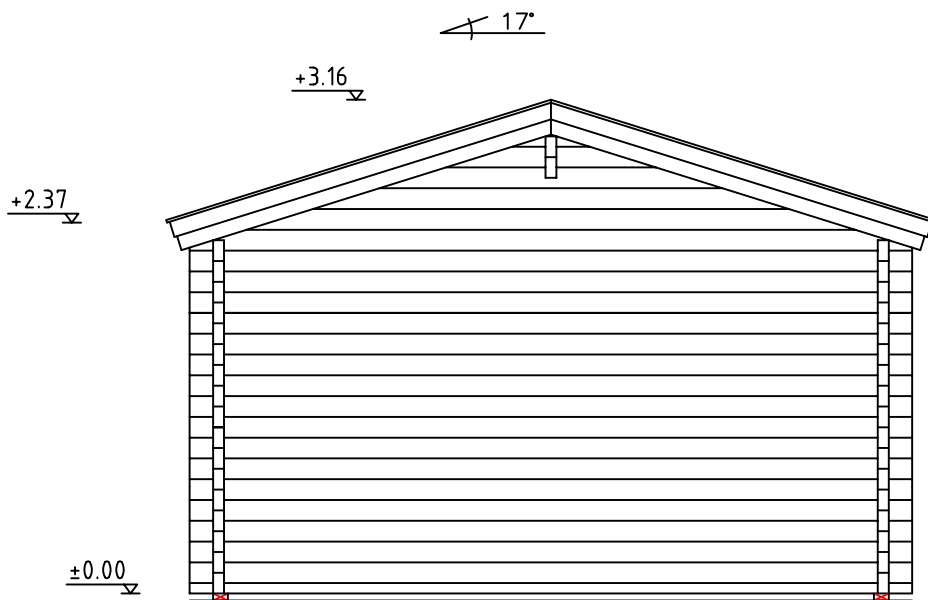
Section -B
