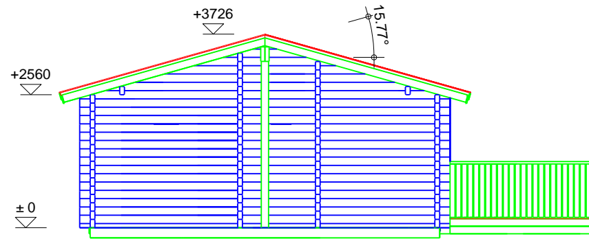
Section-C
