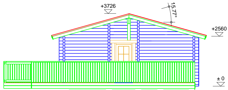
Section-D
