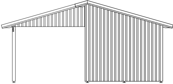
ANSICHT -B
