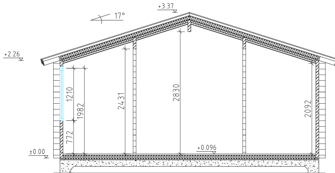
Cross-section A-A
