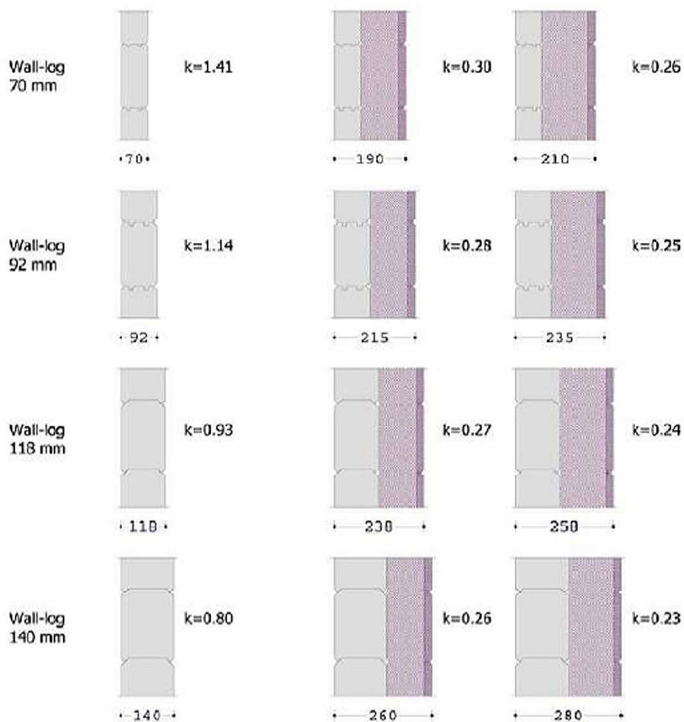
Log-wall with insulation
