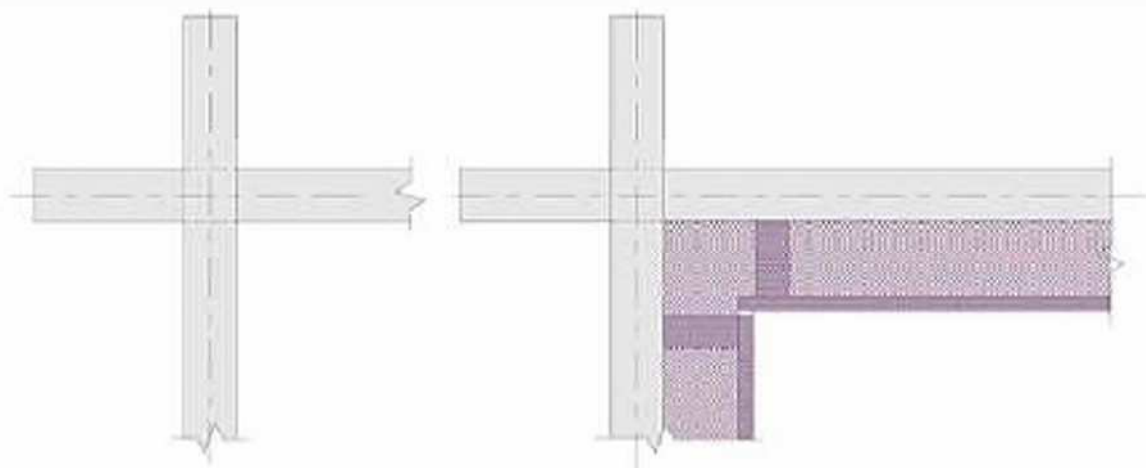
Log-wall with insulation
